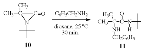
Scheme 6. Reaction of 1- tert -butyl-3,3-dimethylaziridinone with benzylamine.
