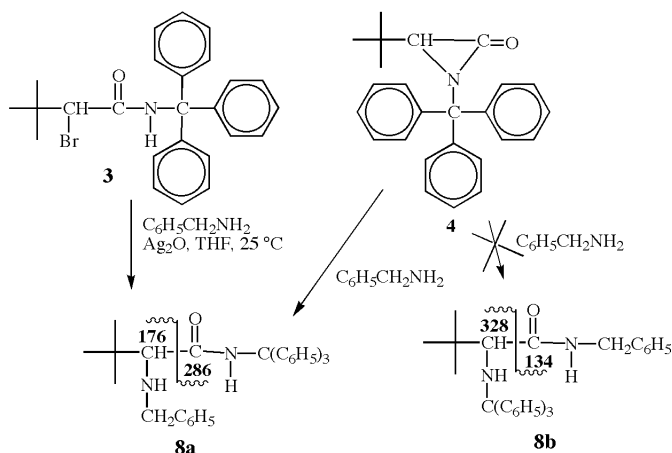
Scheme 5. Reaction of \alpha -lactam 4 with benzylamine and an independent synthesis of 8a .
