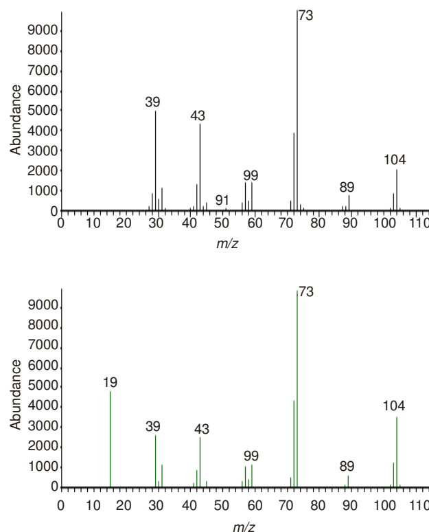
Fig. 2. Mass spectra of the product and the standard trimethyl borate under the same condition
