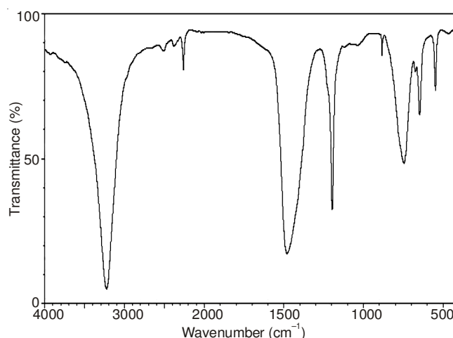
Fig. 7. Infrared spectra of pure boric acid
