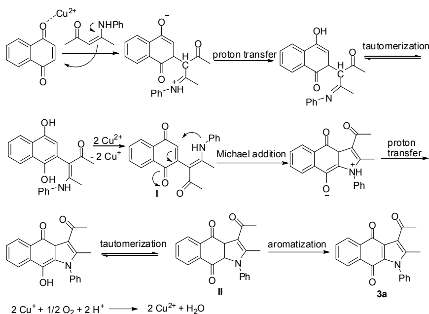
Scheme 1. Plausible Reaction Pathway
