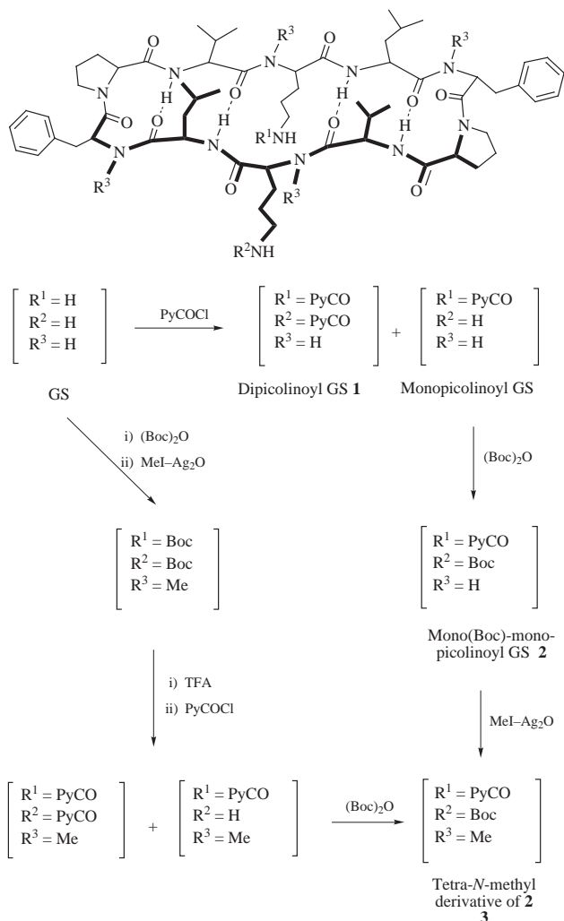
Scheme 1 Preparation of picolinoyl derivatives [Orn(PyCO) 2.2 ]GS 1 , [Orn(Boc) 2 ,Orn(PyCO) 2 ] 2 and [MeOrn(Boc) 2 ,MeOrn(PyCO) 2 ,D-MePhe 4,4 ]GS 3 from gramicidin S (GS).
