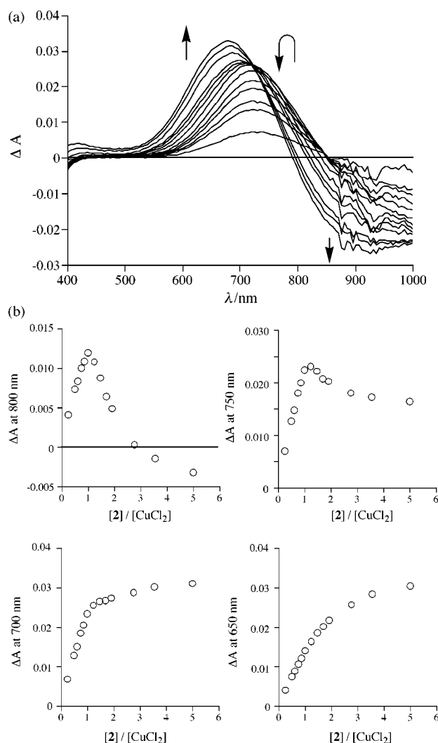
Fig. 4 Absorption spectral change of CuCl 2 in MeOH with the addition of the monopicolinoyl derivative 2 (25 °C; [CuCl 2 ] = 1.0 × 10 -3 M, [2] = 0.26–5.0 × 10 -3 M). (a) Difference spectra are given. Δ A refers to the absorbance of the solution less the absorbances of the component solutions of CuCl 2 and compound 2 at the corresponding concentrations. (b) Plots of Δ A vs. [2]/[CuCl 2 ] at 800, 750, 700 and 650 nm are shown.
