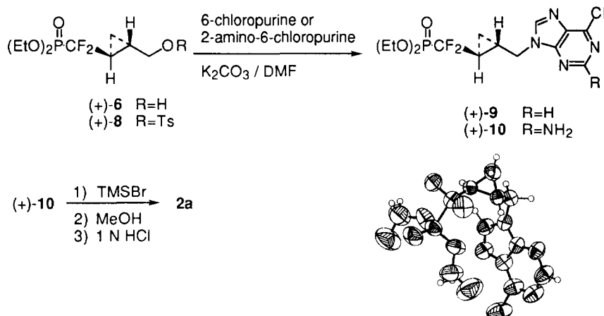
Fig. 1 ORTEP drawing of (+)- 9
