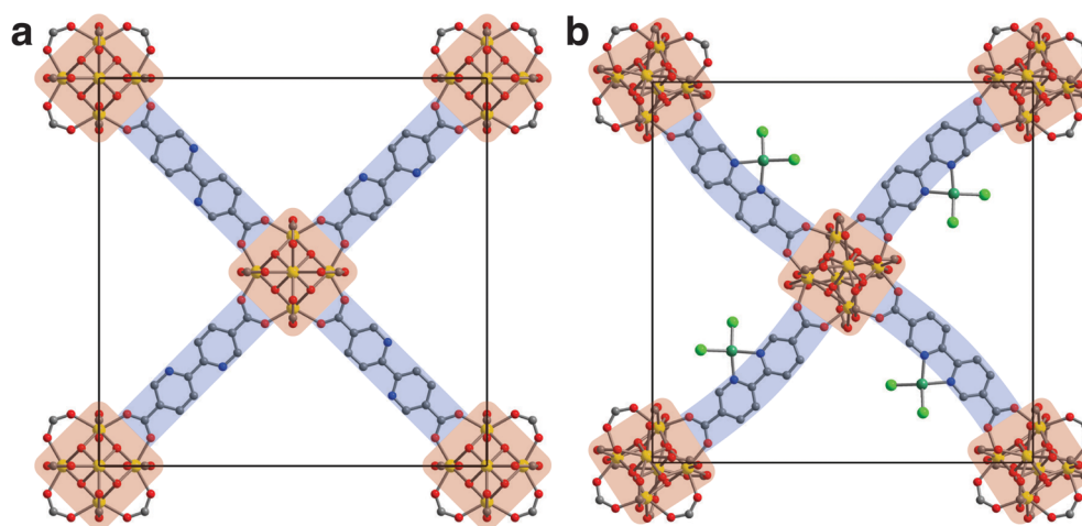
Figure 3. Comparison of the crystal structures of 1 (a) and 1 ·(CuCl 2 ) 5.8 (b) viewed along the [100] direction; unit cell edges are shown as black lines. The bare framework exhibits mirror symmetry along the body diagonals of its unit cell and face-centering translations that relate the zirconium clusters at the ends of each linker. In the metalated structure, the mirror symmetry is removed by the ordering of the linkers, while the face-centering is lost because the clusters at the ends of each linker are tilted in opposite directions.
