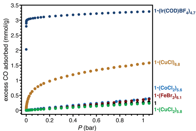
Figure 5. Low-pressure CO adsorption isotherms for 1 , 1\cdot(\text{CuCl}_2)_{5.8} , 1\cdot(\text{CuCl})_{6.8} , 1\cdot(\text{CoCl}_2)_{5.5} , 1\cdot(\text{FeBr}_2)_{6.1} and 1\cdot(\text{Ir}(\text{COD})\text{BF}_4)_{4.8} at 298 K.
