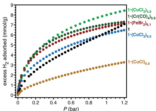
Figure 4. Low-pressure \text{H}_2 adsorption isotherms for 1 , 1\cdot(\text{CuCl}_2)_{5.8} , 1\cdot(\text{CuCl})_{6.8} , 1\cdot(\text{CoCl}_2)_{5.5} , 1\cdot(\text{FeBr}_2)_{6.1} , and 1\cdot(\text{Cr}(\text{CO})_4)_{5.6} at 77 K.
