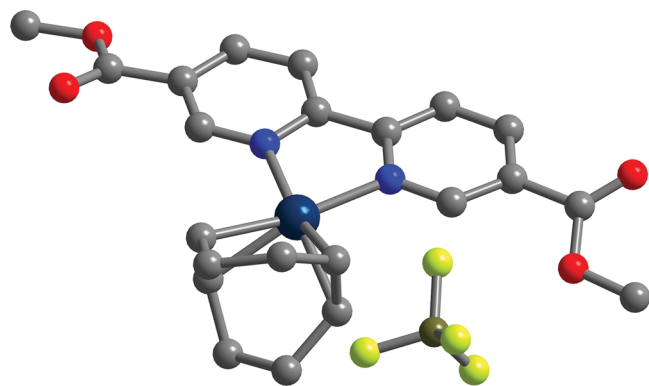
Figure 6. Crystal structure of 3 , the molecular analog of 1 ·(Ir(COD)BF 4 ) 4.7 as determined by single-crystal X-ray diffraction. Dark blue, yellow green, olive green, red, blue, and gray spheres represent Ir, F, B, O, N, and C atoms, respectively; H atoms are omitted for clarity.
