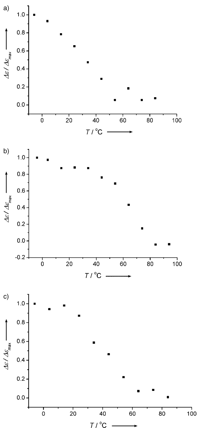
Figure 9. Temperature dependence of the CD effect in spectra of 1 mM solutions of compounds 3 (A), 4b (B), and 7b (C) in dodecane. The fraction of the maximum ellipticity remaining is plotted against temperature.
