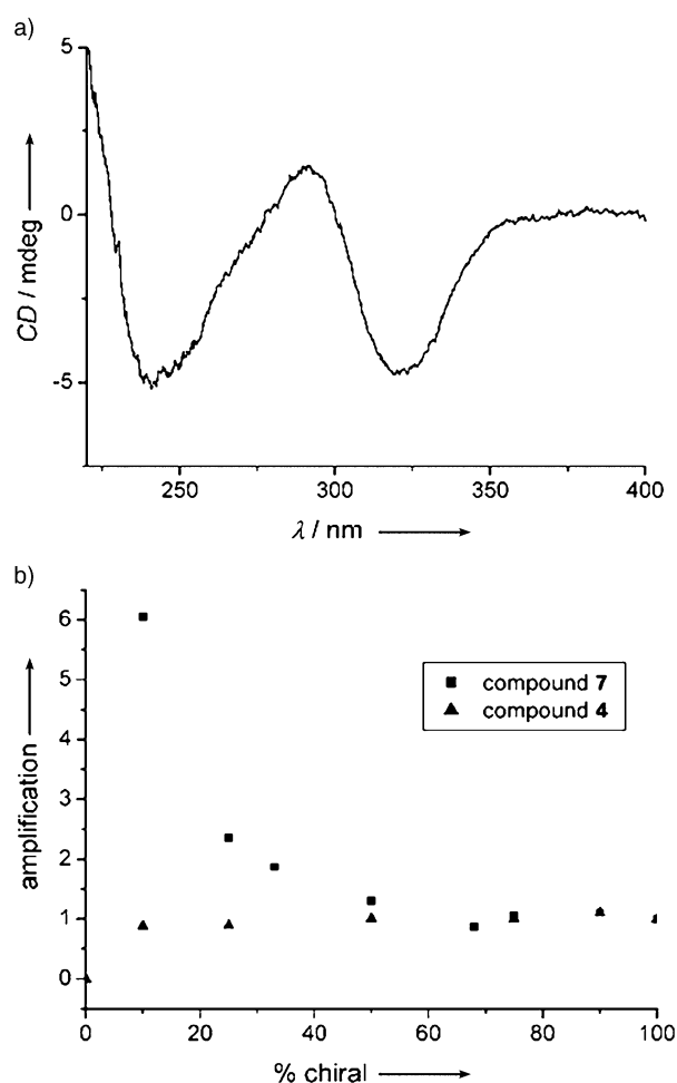
Figure 8. a) CD spectrum of a 1 mM dodecane solution of compound 7b at -6^{\circ}\text{C} . b) “Sergeants and soldiers” experiment on mixtures of chiral and achiral compounds at fixed total concentrations of 1 mM in dodecane at -6^{\circ}\text{C} : ( \blacktriangle ) 4a and 4b ; ( \blacksquare ) 7a and 7b . The amplification is defined as the normalized CD effect per chiral molecule versus fraction of chiral compound.
