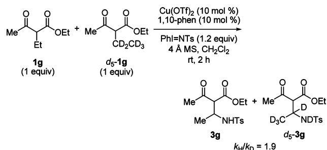
Scheme 6. Measurement of the Deuterium Kinetic Isotope Effect for the Cu(OTf) 2 -Catalyzed Reactions of 1g and d 5 - 1g
