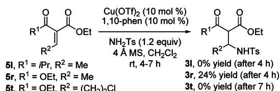
Scheme 4. Cu(OTf) 2 -Catalyzed Reactions of 5l , 5r , and 5t with NH 2 Ts as the Nitrogen Source
