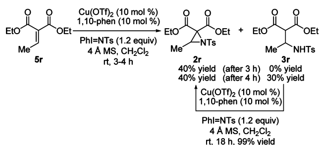
Scheme 2. Cu(OTf) 2 -Catalyzed Reactions of 3r and 5r with PhI=NTs
