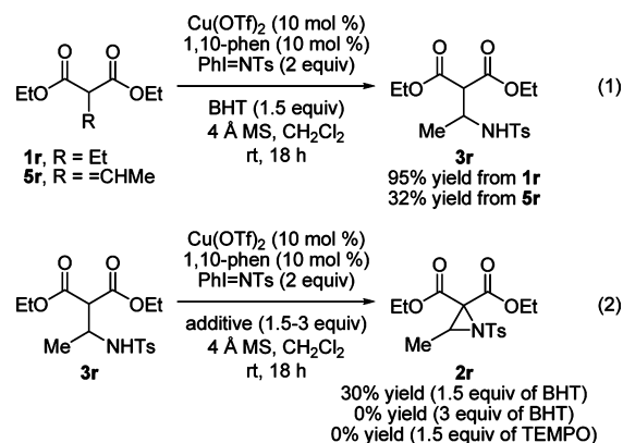
Scheme 5. Cu(OTf) 2 -Catalyzed Reactions of 1r , 3r , and 5r in the Presence of a Radical Scavenger
