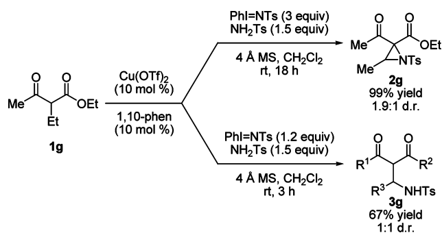
Scheme 3. Cu(OTf) 2 -Catalyzed Reactions of 1g with PhI=NTs in the Presence NH 2 Ts
