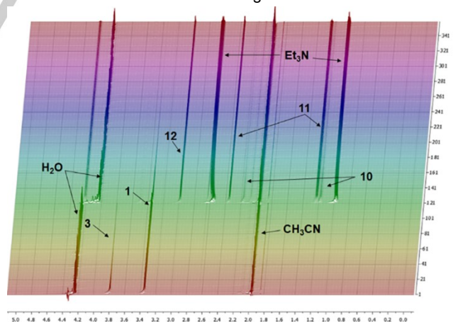
Figure 2. ^1\text{H} NMR reaction profile for mesyl azide generation at 25\text{ }^\circ\text{C} followed by subsequent diazo transfer, showing characteristic signals for mesyl chloride ( 3 ), mesyl azide ( 1 ), methanesulfonamide ( 12 ), ethyl 2-diazoacetoacetate ( 11 ), ethyl acetoacetate ( 10 ), triethylamine, acetonitrile and water.
