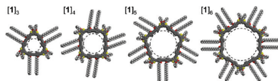
Figure 1. Molecular models of the cyclooligomers [1]_n , n = 3–6 . Maximum diameters of circles fitted into the cores: [1]_3 , 1.5 nm; [1]_4 , 2.4 nm; [1]_5 , 3.0 nm; [1]_6 , 3.8 nm.
