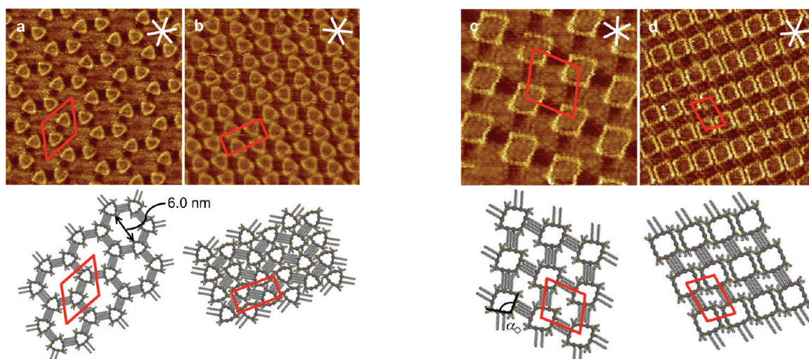
Figure 3. STM images and molecular models of the cyclooligomer patterns at the TCB/HOPG interface. (a), (b) [1]_3 (a: c = 10^{-6} M, 40.0 \times 40.0 nm 2 , V_S = -1.0 V, I_t = 4 pA, thermally annealed for 30 s at 60 °C; p6mm , a = 8.2 \pm 0.2 nm, b = 8.1 \pm 0.2 nm, \gamma(a,b) = 60 \pm 2^\circ ; b: c = 10^{-5} M, 35.5 \times 35.5 nm 2 , V_S = -1.0 V, I_t = 4 pA, thermally annealed for 1 min at 60 °C; p2mg , a = 7.8 \pm 0.2 nm, b = 3.7 \pm 0.1 nm, \gamma(a,b) = 90 \pm 2^\circ ), and (c), (d) [1]_4 (c: c = 10^{-6} M, 29.5 \times 29.5 nm 2 , V_S = -0.8 V, I_t = 30 pA, thermally annealed for 1 min at 80 °C; p2 , a = 5.6 \pm 0.2 nm, b = 5.4 \pm 0.2 nm, \gamma(a,b) = 73 \pm 2^\circ ; d: c = 10^{-5} M, 34.9 \times 34.9 nm 2 , V_S = -1.2 V, I_t = 10 pA, thermally annealed for 1 min at 60 °C; p2 , a = 5.6 \pm 0.2 nm, b = 3.8 \pm 0.1 nm, \gamma(a,b) = 76 \pm 2^\circ ). The unit cells are shown in red; the white lines indicate the HOPG main axis directions. 5
