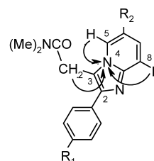
Chart 3. Selected HMBC Correlations for 1 and 2 (Solvent: DMSO- d 6 )
