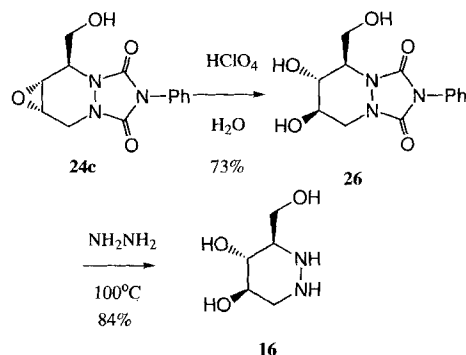
Scheme 9. Stereoselective synthesis of 26 and its hydrazinolysis to 1-azafagomine ( 16 ).
