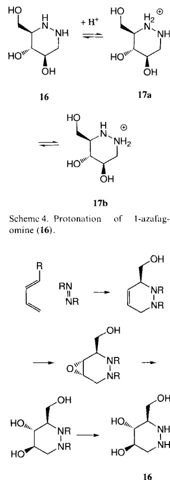
Scheme 5. Strategy for the synthesis of 1-azafagomine ( 16 ).
