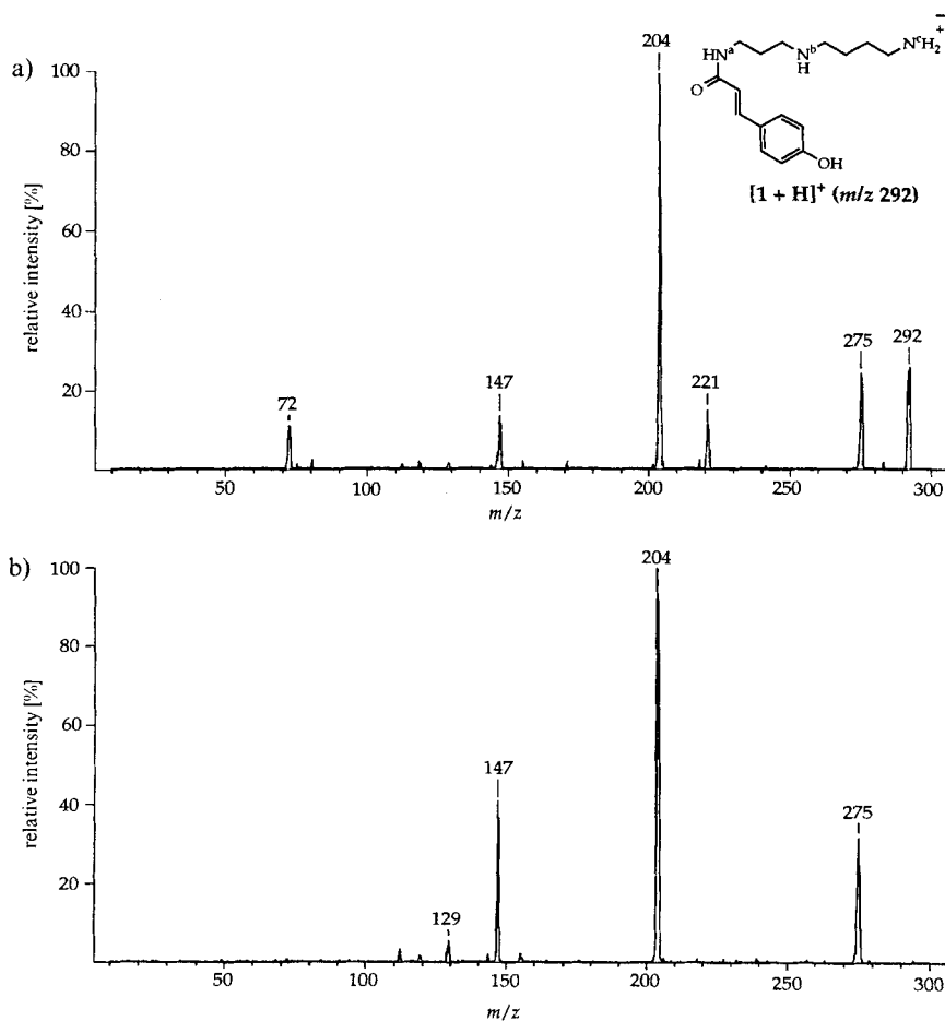
Fig. 1. a) ESI-MS for [ 1 + H] + ( m/z 292). b) ESI-MS/MS/MS for its daughter ion m/z 275
