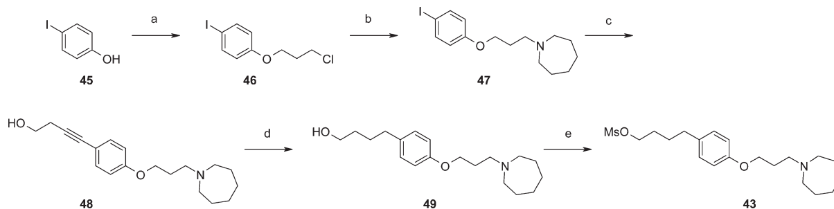
Scheme 8 a
