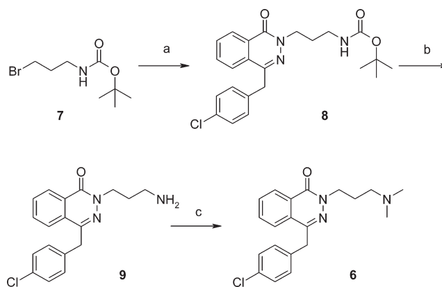
Scheme 2 a
