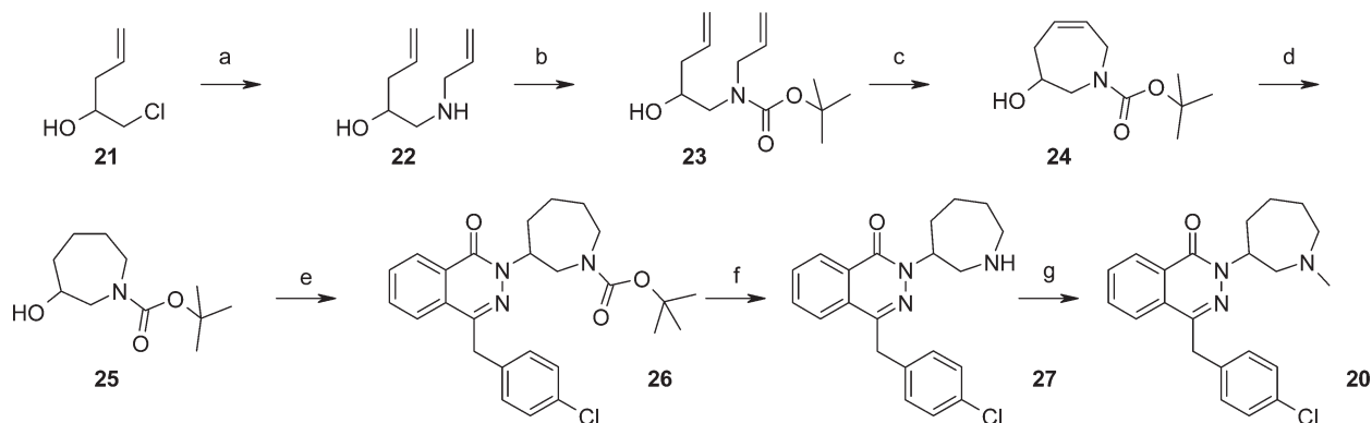
Scheme 5 a
