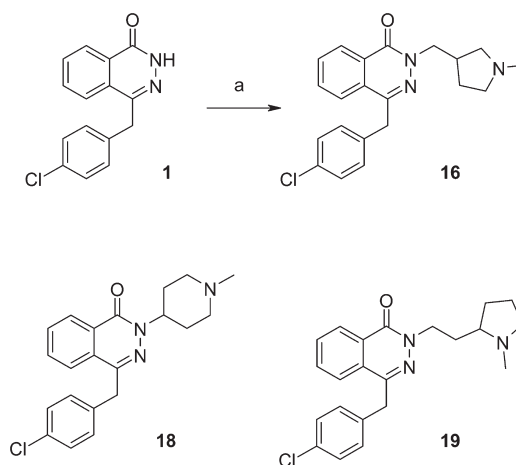
Scheme 4 a
