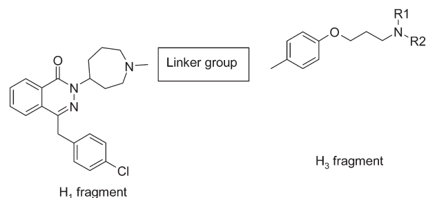
Chart 3. Strategy for Dual H 1 H 3 Antagonism on a Single Ligand
