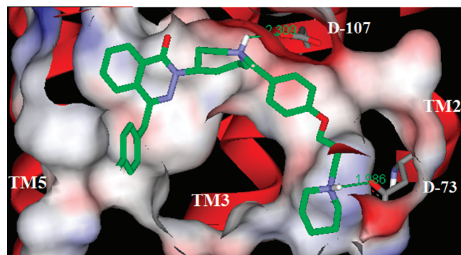
Figure 2. One of the low-energy conformations of the extended azelastine ligand 40 docked into the homology model of H 1 .
