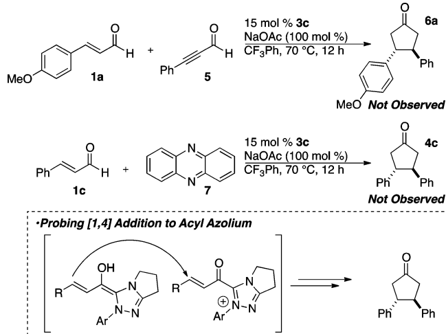
Scheme 2. Control Experiments
