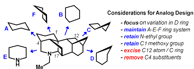
Figure 2. Ring labeling and analog design considerations.
