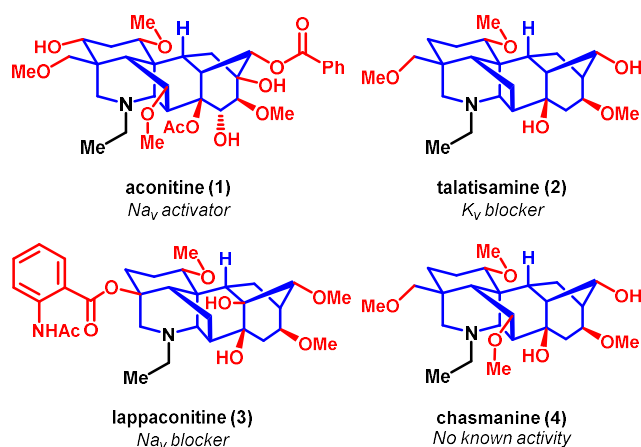
Figure 1. Selected examples of diterpenoid alkaloids.
