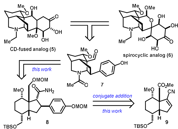
Figure 3. Retrosynthesis of two classes of aconitine analogs.
