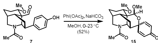
Scheme 2. Oxidative dearomatization of 7 to build spirocyclic scaffold.
