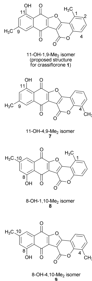
Fig. 4 Hydroxy-dimethyl-6 H -naphtho[2',3':4,5]furo[3,2- c ]chromene-6,7,12-triones: structure reported for crassiflorone 1 , and three regioisomers 7–9 thereof, possible structures for the natural product.
