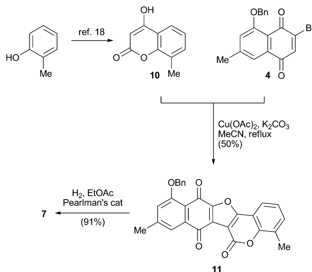
Scheme 2 Synthesis of the 11-hydroxy-4,9-dimethyl furocoumarin naphthoquinone 7 .
