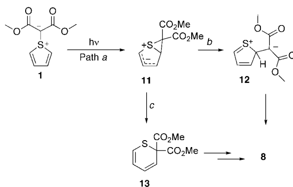
SCHEME 2. Potential Mechanistic Pathways for Formation of 8 on Photolysis of 1
