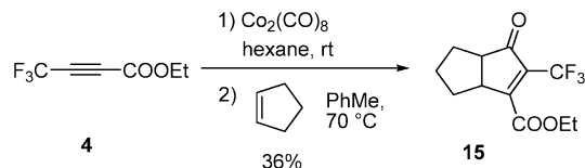
Scheme 6. Stoichiometric PKR of 4 with Cyclopentene
