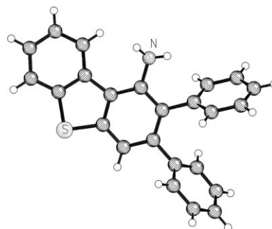
Figure 3. Molecular structure of 20 as obtained by X-ray diffraction (SCHAKAL plot). [7]
