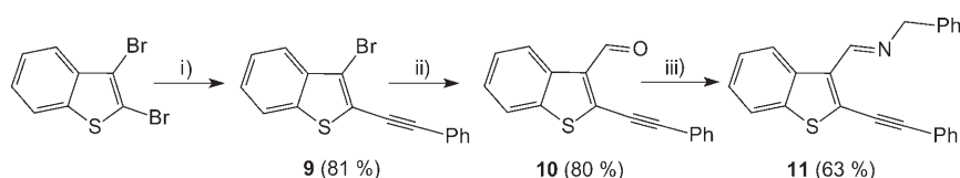
Scheme 3. Reagents and conditions: i) PhCCH, [Pd(Ph 3 P) 2 Cl 2 ], CuI, Et 3 N, 20°C; ii) 1. n BuLi, 2. DMF; iii) PhCH 2 NH 2 , CH 2 Cl 2 , molecular sieves.
