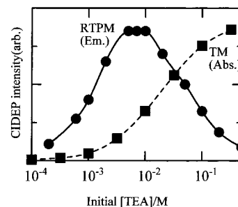
Figure 5. Kinetic simulation of the CIDEP intensities at t = 1.5 \mu s as a function of initial concentration of TEA. Emissive polarization due to RTPM is indicated by the solid line and absorptive polarization due to TM is indicated by the broken line.
