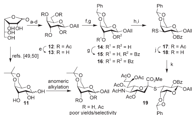
Scheme 2. Synthesis of protected thiosialosyl galactoside 19 . a) NaBH 4 , H 2 O, H + resin, 0°C; b) Ac 2 O, pyridine; c) 45% HBr/HOAc, CH 2 Cl 2 , 0°C→RT; d) AlOH, Drierite, Hg(CN) 2 , HgBr 2 ; e) cat. NaOMe, MeOH, 73% over 3 steps; f) PhCH(OMe) 2 , DMF/MeCN, cat. p TSA-H 2 O, 73%; g) pyridine, BzCl, CH 2 Cl 2 , 0°C, 94%; h) Tf 2 O, pyridine, CH 2 Cl 2 , -20→-5°C; i) KSAc, DMF, 50°C, 94% over 2 steps; j) hydrazine acetate, DMF, 98%; k) NaH, DMF, then 6 , Kryptofix 21, 90%.
