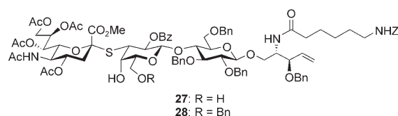
Figure 3. Potential intermediates in the chemical synthesis of S-GM 2 .
