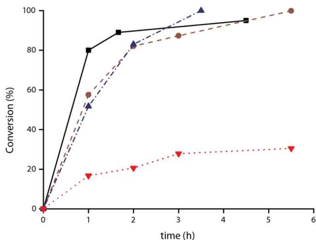
Figure 2. Kinetic plots for reactions with different catalysts (2.5 mmol %) under optimal conditions for each: ■, 7 in methanol, using ultrasonication (taken from Figure 1); ●, free DMAN in methanol; ▲, polymer-bound DMAN (S2) in toluene; ▼, without catalyst in methanol.
