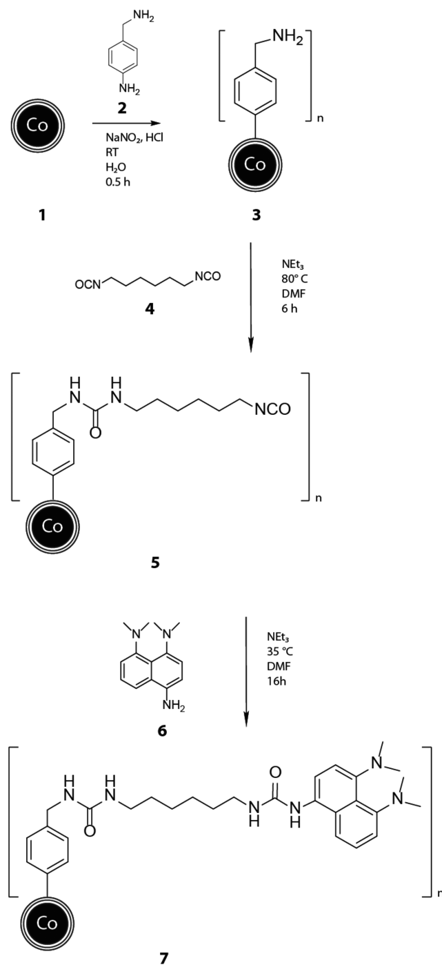
Scheme 1. Synthesis of Immobilized Magnetic Superbase 7 a
