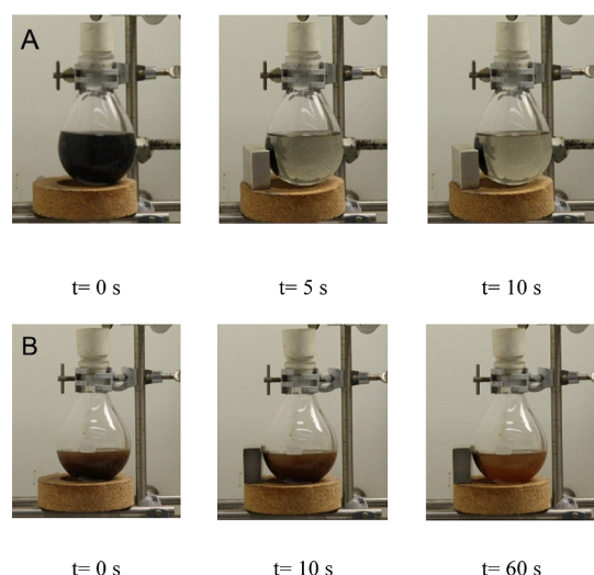
Figure 3. Recovery of organic base bound to magnetic nanoparticles using a low-cost external magnet. Model system in H 2 O; same particle concentration as used in all experiments (0.7 mg mL -1 ). A, metal-based reagents derived from Co/C; B, silica-coated Fe 3 O 4 . Note the different times above and below.
