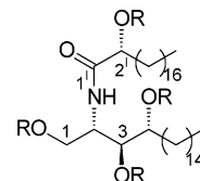
3 : R = H; 3a : R = Ac
