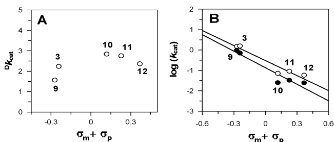
Figure 3. Flavin substituent effects on Dk_{\text{cat}} . Reactions with IPP and (R)-[2- 3 H]-IPP (○ and ● circles, respectively, in panel B) were carried out under pseudo-first-order conditions as described in the Supporting Information. (A) Calculated Dk_{\text{cat}} from the data in panel (B). (B) Hammett plots: \rho = -2.5(4) and -2.7(5) for IPP and (R)-[2- 3 H]-IPP, respectively.
