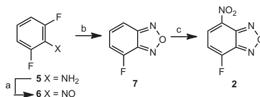
Scheme 1. Reagents and conditions: (a) mCPBA, DCM, 0 °C to 23 °C, 2 h, 100%; (b) \text{NaN}_3 , DMSO, 23 °C, 2 h; (c) \text{NaNO}_3 , \text{H}_2\text{SO}_4 (aq), 0 °C, 3 min, 24% over two steps.
