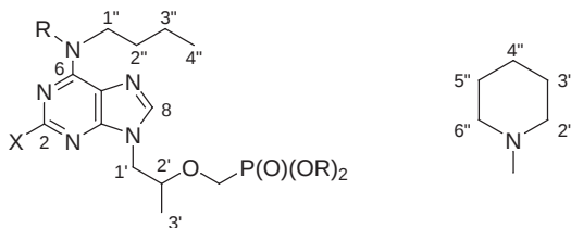
FIG. 1 General numbering scheme for assignment of NMR signals
