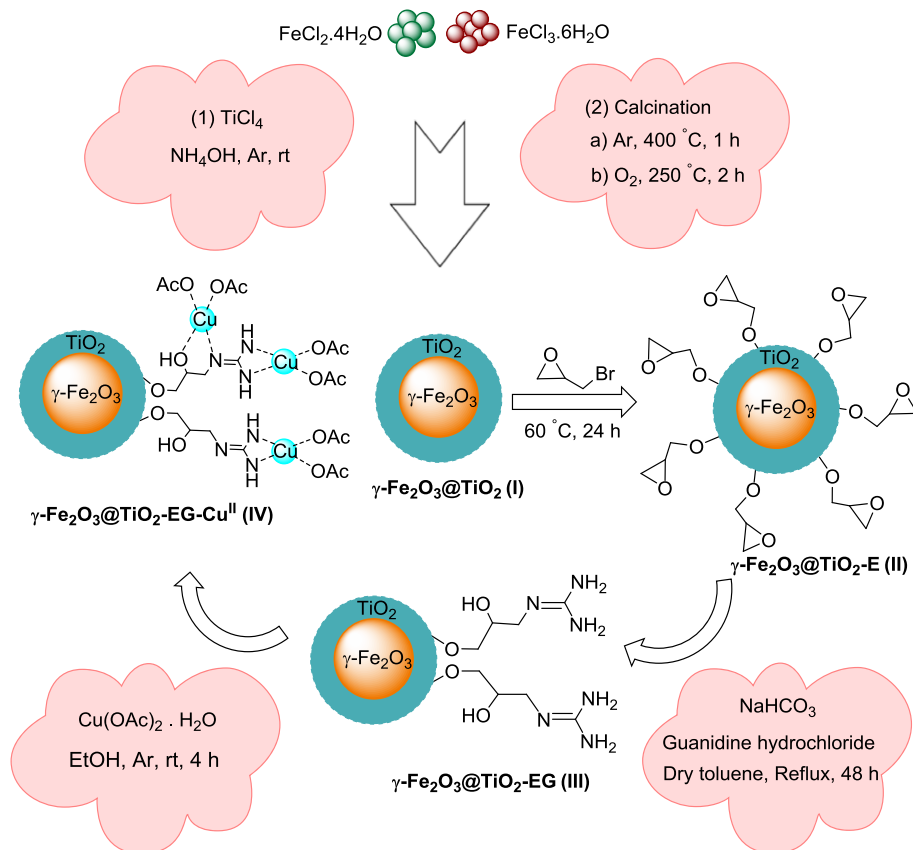
SCHEME 1 Overview of \gamma\text{-Fe}_2\text{O}_3\text{@TiO}_2\text{-EG-Cu(II)} preparation
