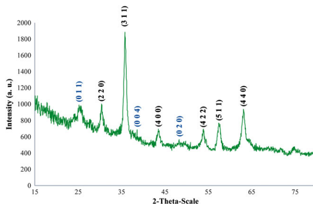
FIGURE 2 XRD pattern of \gamma\text{-Fe}_2\text{O}_3@TiO_2
