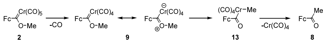
Scheme 3.
