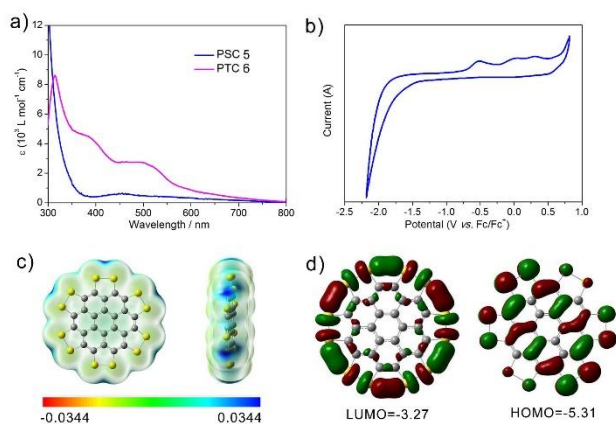
Figure 4. (a) UV/Vis absorption spectrum of PSC 5 (blue) and PTC 6 (pink) in NMP ( 5 \times 10^{-6} M). (b) Cyclic voltammogram of 5 in THF solution of \text{Bu}_4\text{NPF}_6 (0.1 M) with a scan rate of 50 mV/s. (c) Electrostatic potential of 5 . (d) Molecular orbitals of 5 by DFT calculation (B3LYP/6-31G (d, p)). Left: LUMO; right: HOMO, the orbital energies are given in eV.
