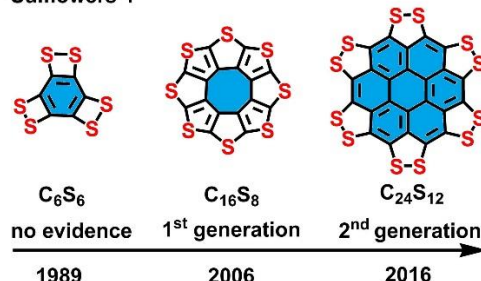
Figure 1. “Sulflower” molecules: (left) persulfurated benzene (C 6 S 6 ); (middle) fully sulfur-substituted circulene (C 16 S 8 ); (right) persulfurated coronene (C 24 S 12 ).
