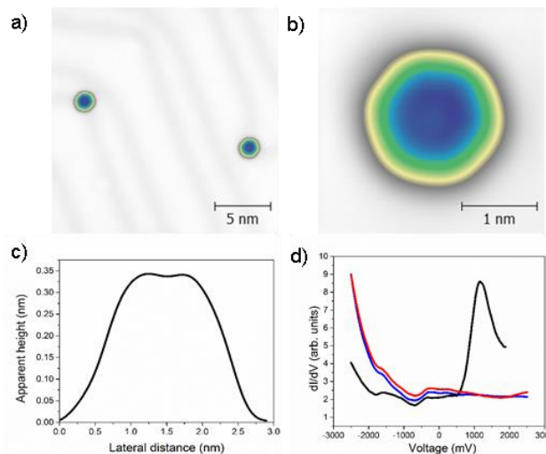
Figure 3. Low-temperature STM characterization of single PSC 5 molecules on the Au (111) surface. (a) STM image showing two PSC 5 molecules adsorbed on an Au (111) terrace at the kink sites ( I = 20 pA, U = 0.7 V); (b) STM image of a PSC 5 molecule ( I = 20 pA, U = 0.5 V); (c) Line scan taken along the molecule in (b); (d) dI/dV spectra of the molecule in (b): bare Au surface (blue curve), center of the molecule (red curve), edge of the molecule (black curve).
