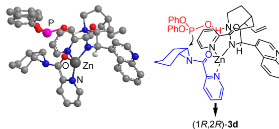
Figure 3. Proposed transition state for the reaction of 1d with diphenyl phosphite 2 using 4g . H-atoms have been omitted for clarity.
