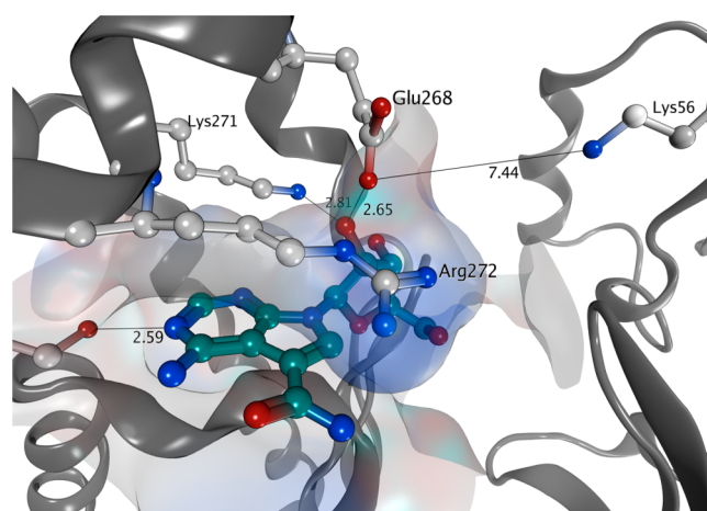
Figure 4. Co-crystal structure of sangivamycin 10 bound to HSP72. PDB 5AQZ, key hydrogen bonding interactions and their distances in Å are indicated. The key salt-bridge interaction between lysine-56 and glutamic acid-268 is absent. Only selected residues are shown and solvent has been omitted for clarity.
