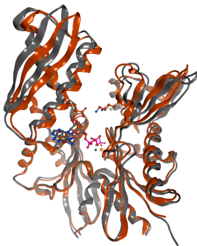
Figure 5. Induced open and induced closed conformations of HSP72. PDB 3ATU and 5AQZ, the copper-colored structure represents the co-crystal structure of ADP/ P_i bound to the HSP72-NBD in the induced closed conformation due to interactions of the phosphate groups through hydrogen bonds with the glycine rich loops and stabilized by the salt-bridge. The gray-colored structure represents the co-crystal structure of sangivamycin 10 bound to the HSP72-NBD. The overlay shows sangivamycin 10 bound to a more open NBD conformation, in which the formation of the Glu-Lys salt-bridge is not possible. Only selected residues are shown and solvent has been omitted for clarity.
