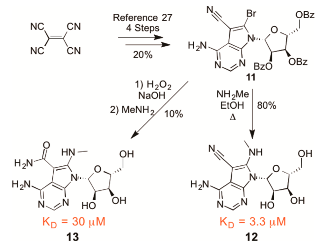
Scheme 1. Natural Product Derived Ligands of HSP70
