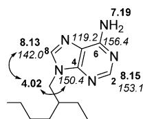
Figure 2. ^1\text{H} ( bold ) and ^{13}\text{C} ( italics ) chemical shifts (in ppm) and key ^1\text{H} – ^{13}\text{C} gHMBC correlations for 4 .
