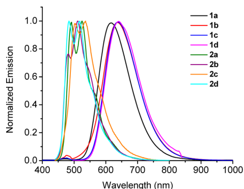
Figure 5. Emission spectra for 1a–d and 2a–d in 1,4-dioxane ( 1\text{--}3 \times 10^{-6} M; \lambda_{\text{ex}} = 476 nm for 1 ; \lambda_{\text{ex}} = 430 nm for 2 ).
