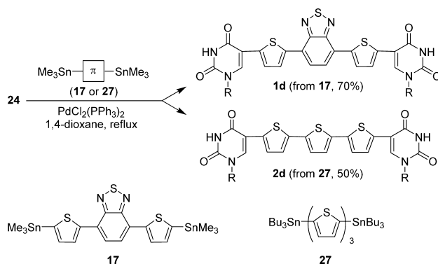
Scheme 7. Synthesis of Uracil-Containing Oligomers 1d and 2d
