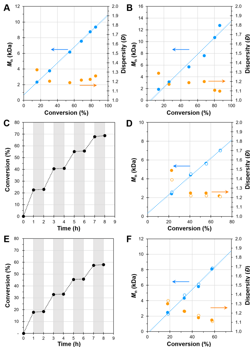
Figure 4. Plots of molecular weight ( M_n , blue) and dispersity ( \bar{D} , orange) as a function of monomer conversion for the polymerization of MMA catalyzed by 3 (A) and 4 (B). Plots of conversion vs time using 3 (C) or 4 (E) (irradiation in white and dark periods in gray) and plots of molecular weight ( M_n , blue) and dispersity ( \bar{D} , orange) as a function of MMA conversion using a pulsed-irradiation sequence and PC 3 (D) or 4 (F) (filled markers are data directly after irradiation while open markers are data directly after the dark period). Conditions for all plots: [MMA]:[DBMM]:[PC] = [1000]:[10]:[1]; 9.35 \mu\text{mol} PC, 1.00 mL dimethylacetamide, and irradiated with UV-light.
