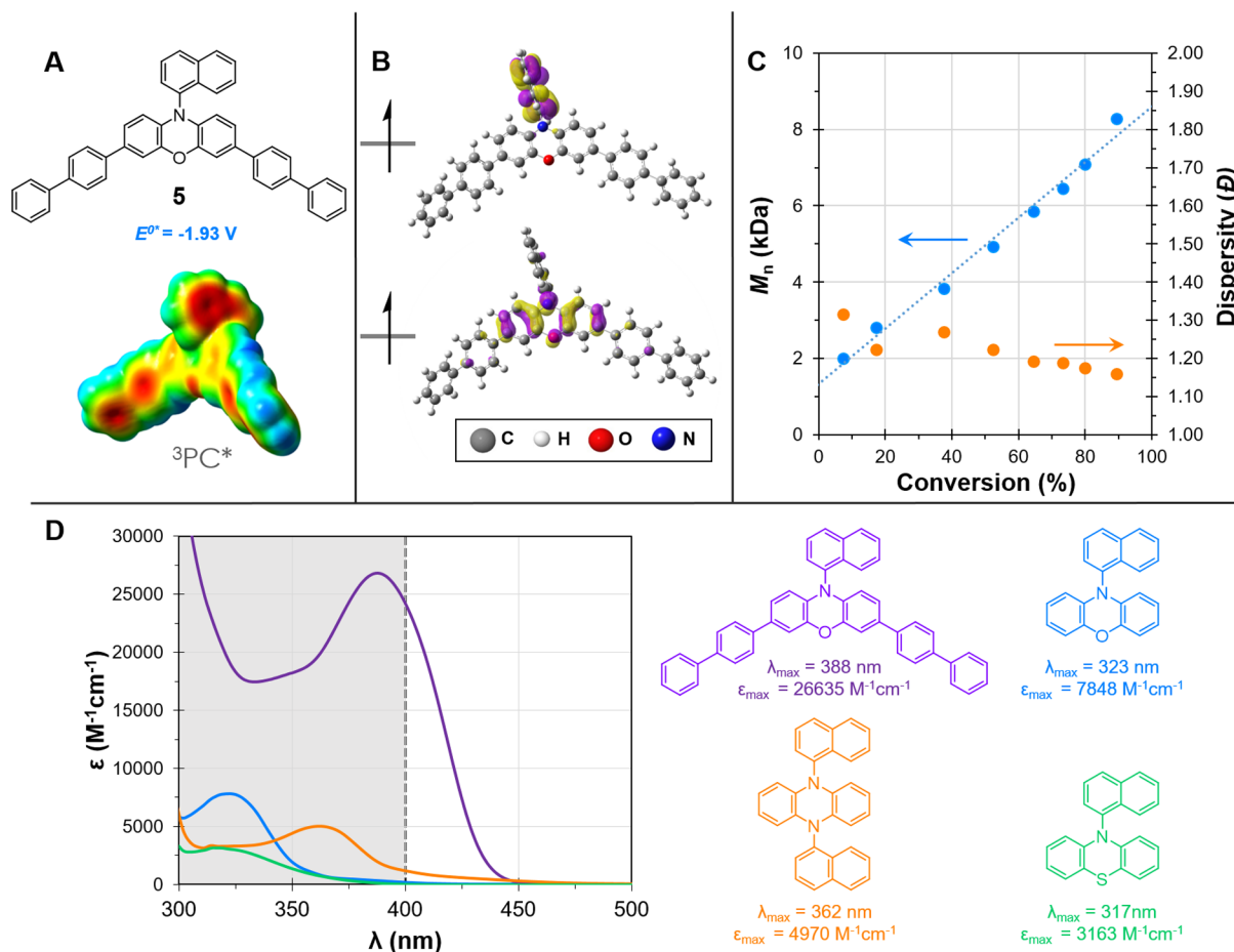
Figure 8. Properties of PC 5. (A) Structure, computed triplet excited state reduction potential, and ESP mapped electron density of ^3PC^* 5. (B) Computed triplet state SOMOs of PC 5. (C) Plot of M_n and \bar{D} as a function of monomer conversion for the polymerization of MMA by PC 5; [MMA]:[DBMM]:[5] = [1000]:[10]:[1]; 9.35 \mu mol PC, 1.00 mL dimethylacetamide, and irradiated with white LEDs. (D) UV-vis spectrum of PC 5 and 1-naphthalene functionalized phenoxazine, dihydrophenazine, and phenothiazine, with color coded structures, and extinction coefficients at their respective \lambda_{max} with the visible absorbance spectrum highlighted in white.
