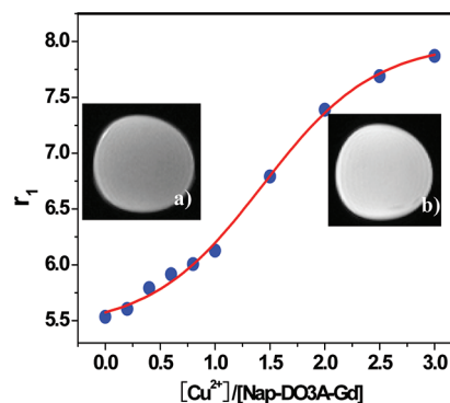
Figure 2. Relaxivity responses of Nap-DO3A-Gd (0.2 mM) to Cu 2+ with various concentrations ( T 1 measurements at a proton frequency of 20 MHz) and T 1 -weighted phantom MRI images: (a) image of only Nap-DO3A-Gd (0.2 mM) in water; (b) image of Nap-DO3A-Gd (0.2 mM) and copper ions (0.6 mM) in water.
