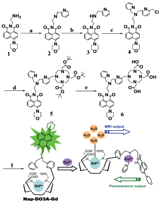
Scheme 1. Synthetic Procedure for Nap-DO3A-Gd a
