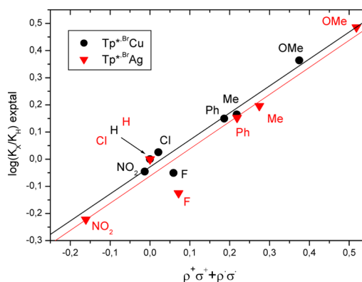
Figure 1. Plot of experimental \log(K_X/K_H) vs calculated \rho^+\sigma^+ + \rho^\bullet\sigma^\bullet (from Table 2) for \text{Tp}^{*,\text{Br}}\text{M} ( M = \text{Cu, Ag} ).
