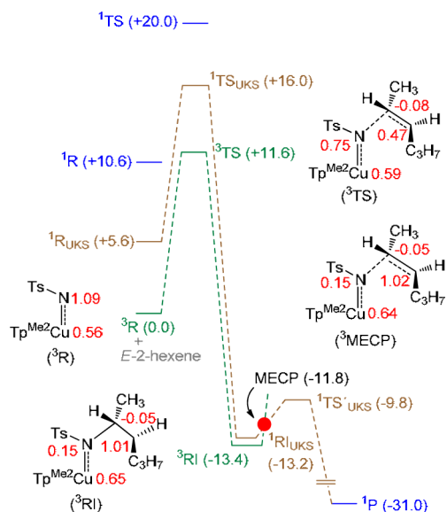
Scheme 9. Computed Free Energy Profiles for Aziridination of E -2-Hexene Catalyzed by \text{Tp}^{\text{Me}_2}\text{CuN-Ts}^a
