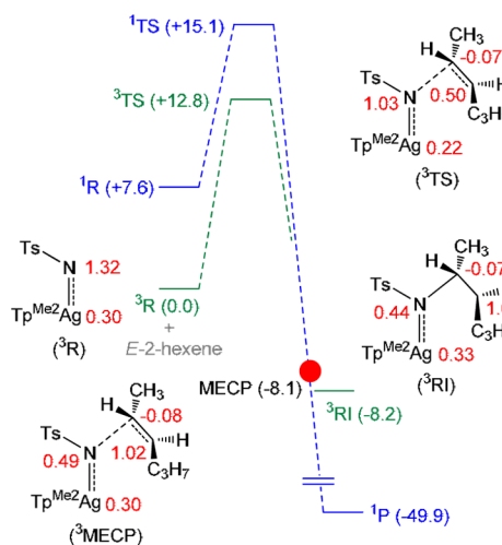
Scheme 8. Computed Free Energy Profiles for the Aziridination of E -2-Hexene Catalyzed by \text{Tp}^{\text{Me}_2}\text{AgN–Ts}^a
