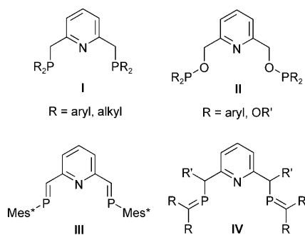
Figure 2. PNP-pincer ligands with different electronic properties.
