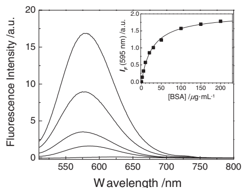
Figure 2. Emission spectra of 1c in the presence of various amounts of BSA. BSA concentrations were 0, 1, 2, 5, and 10 \mu\text{g/mL} from the bottom while SDS concentration was kept constant as 0.005% in 1.5% acetic acid solution. Protein–SDS complex solutions were made by diluting 4 mg/mL BSA stock solution in 1% SDS, which was boiled for 10 min at 95 ^{\circ}\text{C} for complete denaturation of the protein. Inset shows the titration curve of 1c with respect to BSA concentration. [ 1c ] = 1 \mu\text{M} . K_d = 30 \mu\text{g/mL} .
