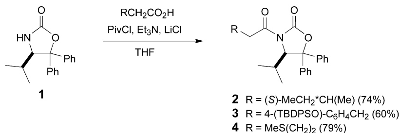
Scheme 1. Acylation of ( R )-DIOZ
