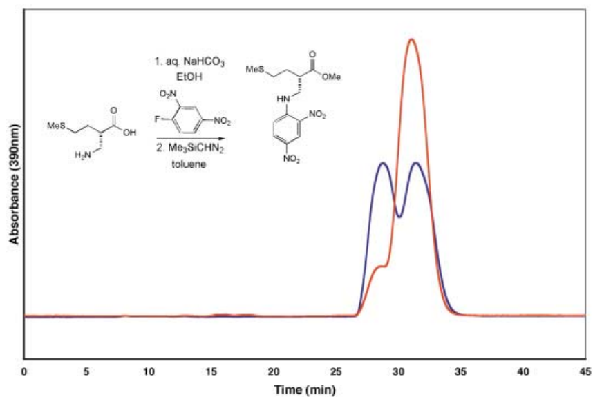
Fig. 3. Determination of enantiomer purity of \beta^2\text{hMet} by HPLC, by using the chiral stationary phase Daicel Chiralpack OD-H
