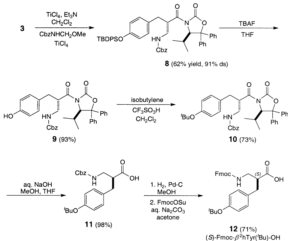
Scheme 3. Preparation of (S)-N-Fmoc- \beta^2 hTyr( t Bu)-OH
