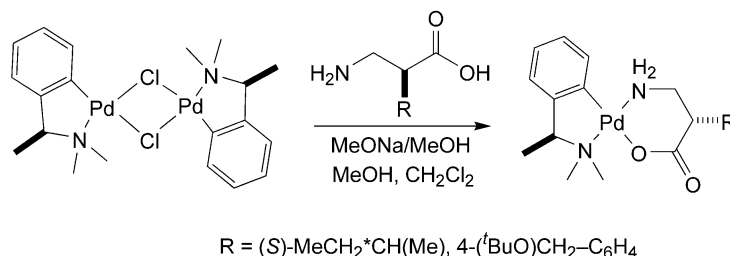
Scheme 5. Preparation of Pd Complexes of \beta^2 -Amino Acids for Determination of Enantiomeric Purity
