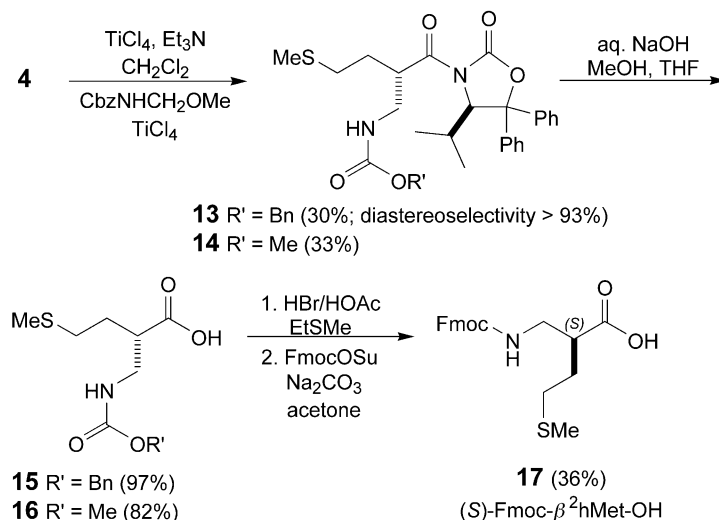
Scheme 4. Preparation of (S)-N-Fmoc- \beta^2 hMet-OH
