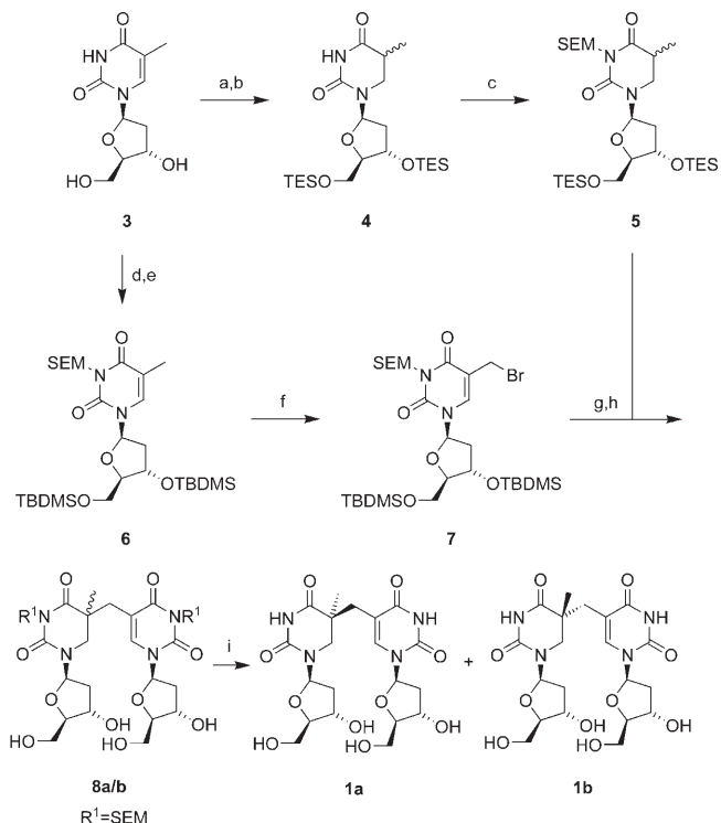
Scheme 3. Synthesis of the substrates with open backbones ( 1a/b ) starting with thymidine 3 . Reagents and conditions: a) \text{Rh}/\text{Al}_2\text{O}_3 , \text{H}_2 , \text{MeOH}/\text{H}_2\text{O} (1:1), RT; b) \text{TESCl} , imidazole, DMF, RT, 88%; c) \text{SEMCl} , i\text{Pr}_2\text{NEt} , \text{CH}_2\text{Cl}_2 , RT, 84%; d) \text{TBDMSCl} , imidazole, DMF, RT, 95%; e) \text{SEMCl} , i\text{Pr}_2\text{NEt} , \text{CH}_2\text{Cl}_2 , RT, 72%; f) \text{NBS} , \text{DBPO} , \text{CCl}_4 , 70^\circ\text{C} , 60%; g) \text{LDA} (1.5 equiv), 5 , THF, -78\text{--}0^\circ\text{C} ; h) \text{TBAF} , THF, RT; rp-HPLC separation, 8a : 15%, 8b : 11%; i) \text{SnCl}_4 , DCM, 0^\circ\text{C} , 55% (for 1b : 75%).
