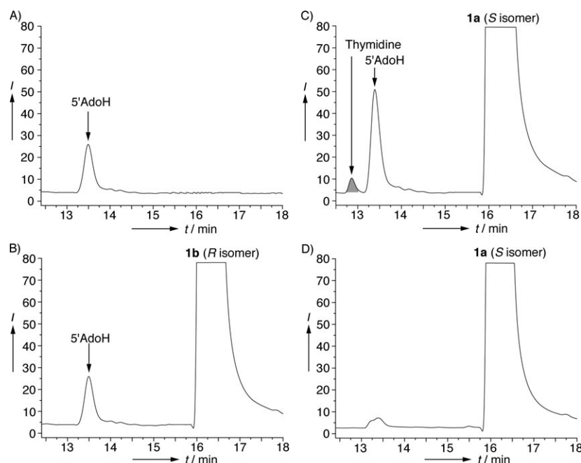
Figure 6. HPL chromatograms of enzymatic studies. The enzyme reaction and rp-HPLC analyses were performed as described in the Experimental Section. A) HPLC analysis of the assay containing 5 nmol splG and SAM. B) HPLC analysis of the assay containing 5 nmol splG, SAM, and the ( R )- 1b . C) HPLC analysis of the assay containing 5 nmol splG, SAM, and ( S )- 1a . Only in this case an additional peak was observed, which was identified as the desired repair product thymidine. D) HPLC analysis of the negative control containing SAM and ( S )- 1a but no splG. In all four chromatograms the y axis shows the intensity of the absorbance at \lambda = 260 nm.
