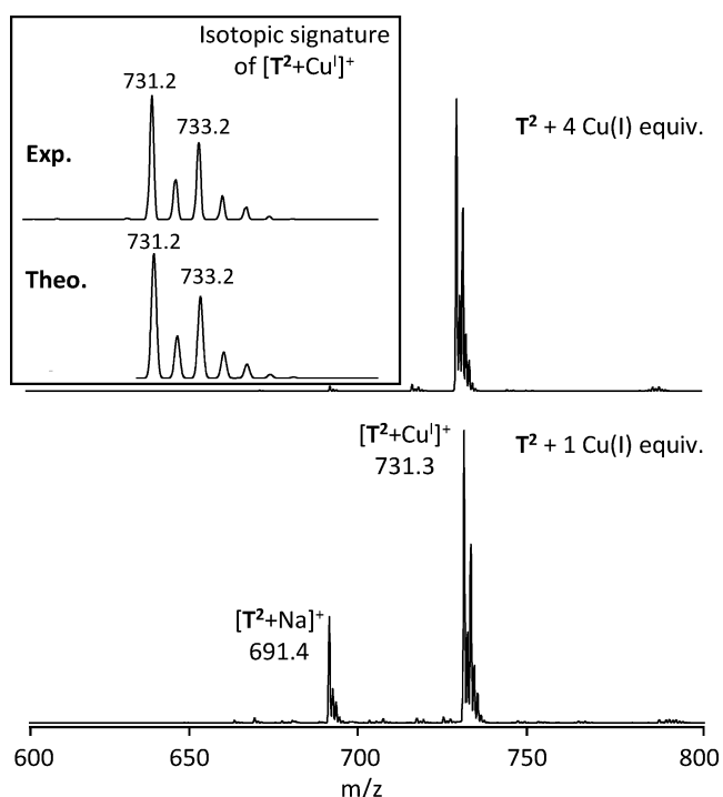
Figure 3. (+) ESI-MS spectra of T 2 (100 \mu M) with equimolar Cu(I) (down) and 4 equiv (top) in water/MeCN (9/1, v/v). Inset shows isotopic patterns (experimental (Exp.) and calculated (Theo.)).
