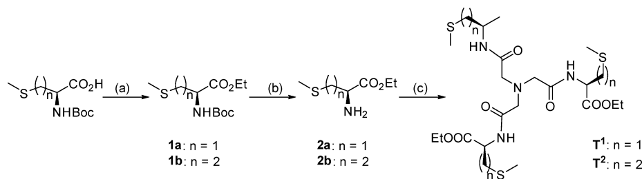
Scheme 1. Syntheses of the Thioether-Based Scaffolds \text{T}^{1,2} a
