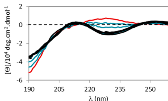
Figure 2. Circular dichroism (CD) titrations of \text{T}^1 (19 \mu\text{M} ) in MeCN/water (1/9, v/v) with Cu(I) (0–2 equiv): (red trace) free \text{T}^1 ; (blue trace) 0.25–0.75 equiv of Cu(I); and (black trace) 1–2 equiv of Cu(I).
