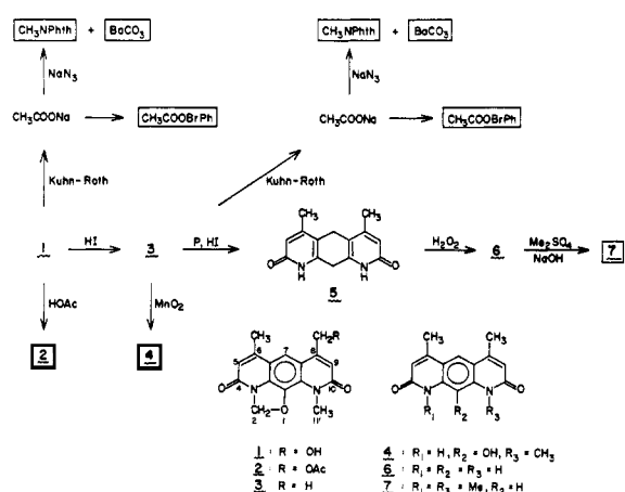
Figure 1. Numbering system employed and degradation scheme for location of the 14 C label in nybomycin ( 1 ); primary reference compounds for counting are enclosed in boxes: Phth = phthaloyl; BrPh = p -bromophenacyl.
