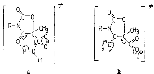
Chart 3. Decarboxylation of the Carboxylate (a) in Aqueous Media and (b) in Micellar Media (R = 3,5-Dichlorophenyl)
