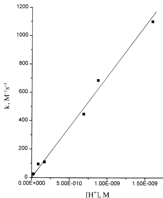
Figure 2. Hydrogen ion dependence on the rate of the thiosulfate/ferrate reaction. Conditions: T = 25.0\text{ }^{\circ}\text{C} , I = 1.0\text{ M} ( \text{NaClO}_4 ), 0.05\text{ M} ( \text{Na} phosphate) buffer.
