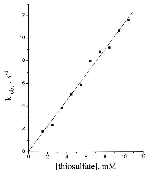
Figure 1. Typical plot of k_{\text{obs}} versus [thiosulfate]. Conditions: pH 8.5, T = 25.0 °C, I = 1.0 M ( \text{NaClO}_4 ), 0.05 M (Na phosphate) buffer.
