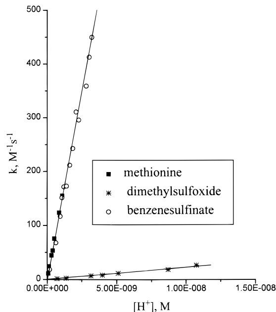
Figure 3. Hydrogen ion dependence on the rate of the S/ferrate reactions. Conditions: T = 25.0 \text{ }^\circ\text{C} , I = 1.0 \text{ M} ( \text{NaClO}_4 ), 0.05 \text{ M} ( \text{Na phosphate} ) buffer.
