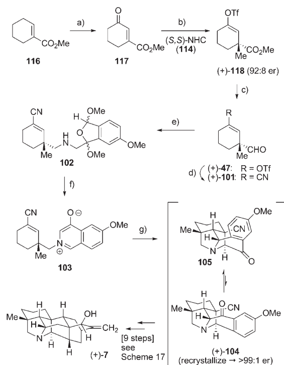
Scheme 19. a) CrO 3 , Ac 2 O, AcOH, CH 2 Cl 2 , 23 °C, 56%; b) 114 , (CuOTf) 2 ·PhH, ZnMe 2 , i BuOMe, 0 °C; add 117 , –30 °C; add Tf 2 O, 0 °C, 88%, 92:08 er; c) DIBAL-H, pentane, –105 °C, 92%; d) Zn(CN) 2 , [Pd(PPh 3 ) 4 ], DMF, 60 °C, 82%; e) 93 , PBu 3 , CH 2 Cl 2 , 23 °C; add (+)- 101 ; add NaBH(OAc) 3 , 82% (3:2 dr); f) 1:10 TFA/CH 2 Cl 2 , 0 °C, 98%; g) [0.32 M], 180 °C, THF, 97%, (+)- 104/105 1:3.6 at equilibrium; recrystallized from i PrOH, 104 92:8 → >99:01 er.
