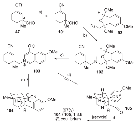
Scheme 16. a) Zn(CN) 2 , [Pd(PPh 3 ) 4 ], DMF, 60°C, 85%; b) 93 , PBu 3 , CH 2 Cl 2 , 23°C; add 101 ; add NaBH(OAc) 3 , 79% (3:3:2:2 dr); c) 1:10 TFA/CH 2 Cl 2 , 0°C, 93%; d) [1.5 M], 180°C, THF, 97%, 104/105 1:3.6 at equilibrium.
