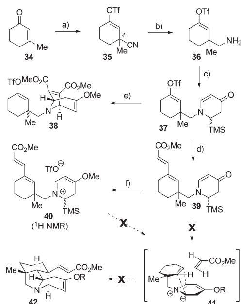
Scheme 6. a) \text{Al}(\text{CN})\text{Et}_2 , \text{PhH} , 23^\circ\text{C} ; ii) TBAT, then \text{Tf}_2\text{O} , 81%; b) DIBAL-H, 0^\circ\text{C} , toluene, \text{NaBH}_4/\text{MeOH} quench, 88%; c) i) \text{TMSCHO} , \text{Et}_2\text{O} , 0^\circ\text{C} ; ii) solvent evaporation, 0^\circ\text{C} ; iii) 27 , \text{ZnCl}_2 , \text{CH}_2\text{Cl}_2 , 0\rightarrow 23^\circ\text{C} , 55%, 1.2:1 dr; d) methyl ( E )-3-tributylstannylacrylate, [\text{Pd}(\text{PPh}_3)_4] , \text{LiCl} , \text{THF} , reflux, 87%; e) \text{MeOTf} , \text{CH}_2\text{Cl}_2 , 23^\circ\text{C} ; DMAD, TBAT, 57%, 1:1 dr; f) \text{MeOTf} , \text{CDCl}_3 , 23^\circ\text{C} , >95%.
