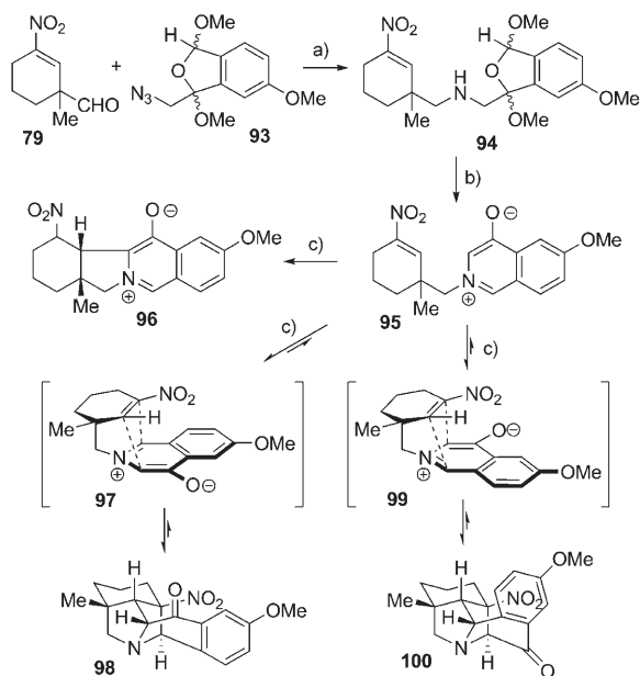
Scheme 15. a) 93 , PBu 3 , CH 2 Cl 2 , 23°C; add 79 ; add NaBH(OAc) 3 , 74% (3:3:2:2 dr); b) 1:10 TFA/CH 2 Cl 2 , 0°C, 98%; c) [0.008 M], PhMe, 90°C (MW wave), 30 min, → 98/100/96 with 4:2:3 isomeric ratio.
