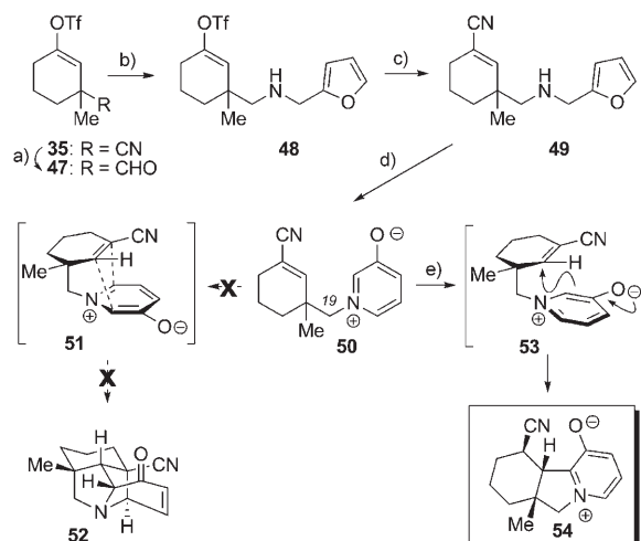
Scheme 8. a) DIBAL-H, 0^\circ\text{C} , \text{PhMe} , 92%; b) furfurylamine·HCl, \text{NaBH}_4 , \text{MeOH} , 3 Å MS, 23^\circ\text{C} , 99%; c) KCN, [18]crown-6, [\text{Pd}(\text{PPh}_3)_4] , \text{PhH} , 75^\circ\text{C} , 75%; d) \text{Br}_2 , 1:1 \text{AcOH/water} , 0^\circ\text{C} , 65%; e) [0.15 M] toluene, 170^\circ\text{C} , 5 d, 73%.
