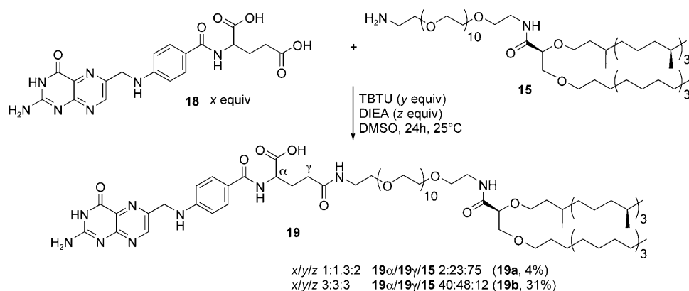
Scheme 7. Synthesis of the targeting folate derivative 19 .
