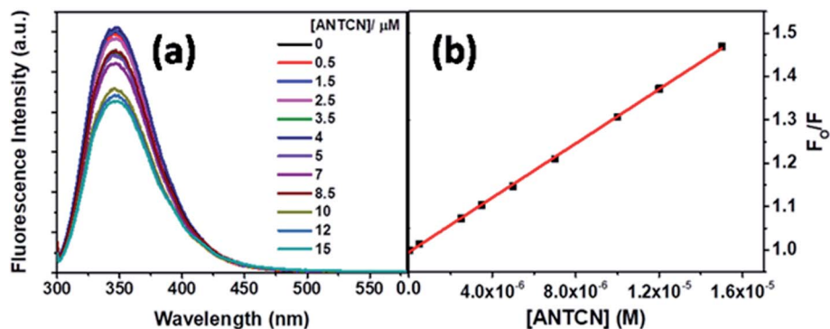
Fig. 14 (a) Fluorescence spectra of Trp residues of BSA and ANTNCN with increasing concentration of ANTNCN, and (b) S-V plot for quenching of Trp fluorescence of BSA by ANTNCN. [BSA] = 5 \mu M, \lambda_{\text{ex}} = 295 nm.
