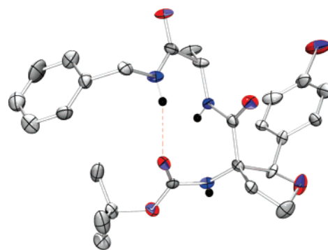
FIGURE 3. X-ray diffraction structure of compound 11 accommodating a \beta turn in the crystal state. The intramolecular i + 3 \rightarrow i hydrogen bond is indicated by a dashed line. Only the amide hydrogen atoms are shown.
