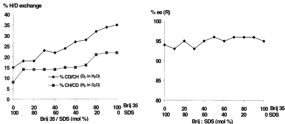
Fig. 4. Influence of SDS–Brij 35 mixtures on the H/D exchange and the enantioselectivity during the hydrogenation or deuteration of methyl (Z)- \alpha -acetamidocinnamate in D 2 O or H 2 O.
