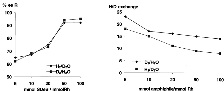
Fig. 5. Influence of different SDeS concentrations on the enantioselectivity and the H/D or the D/H exchange during the hydrogenation or deuteration of methyl (Z)- \alpha -acetamidocinnamate in D 2 O or H 2 O.
