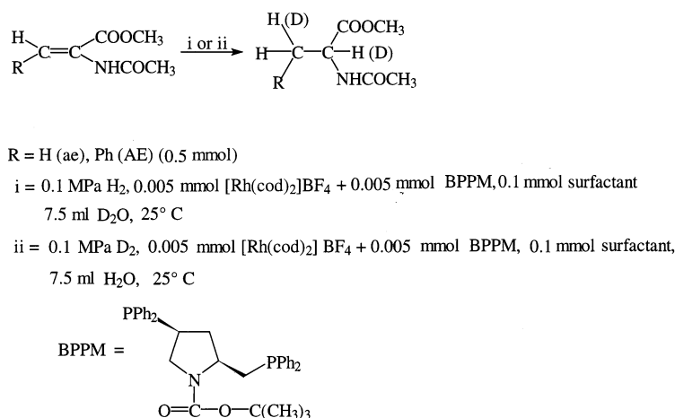
Scheme 1. Asymmetric hydrogenation of unsaturated amino acid derivatives in water.
