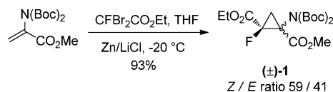
Scheme 1. Cyclopropanation Process Using Zn/LiCl Combination
